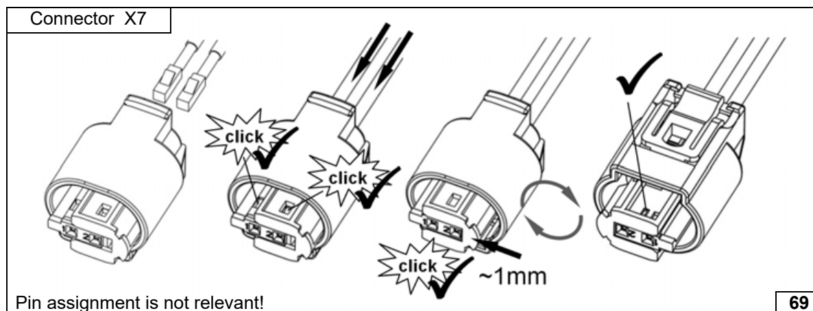
Mounting connector metering pump
